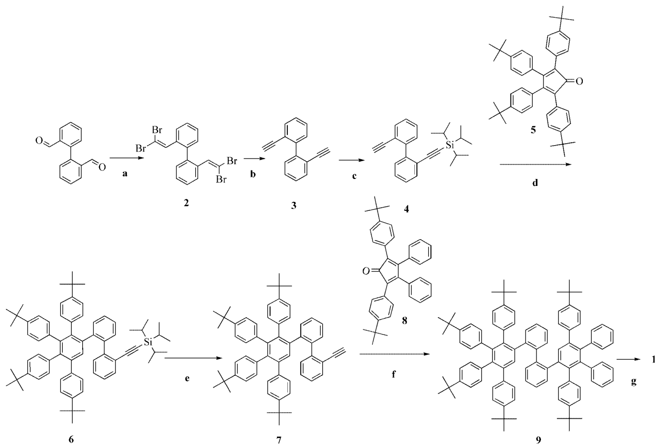
Scheme 1. Route to 1 : (a) \text{CBr}_4 , \text{PPh}_3 , \text{Zn} , \text{CH}_2\text{Cl}_2 (98%); (b) \text{LDA} , \text{THF} (78%); (c) i) n\text{BuLi} , \text{THF} ii) \text{TIPSCl} (57%); (d) Diphenyl ether, microwave irradiation (70%); (e) \text{TBAF/THF} , \text{CH}_2\text{Cl}_2 (84%); (f) Diphenyl ether (60%); (g) \text{FeCl}_3 , \text{CH}_3\text{NO}_2 , \text{CH}_2\text{Cl}_2 , argon bubbling (61%).
