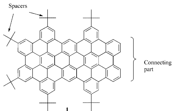
Figure 2. Supracene 2D lander with polyaromatic main board and tert -butyl spacers.
