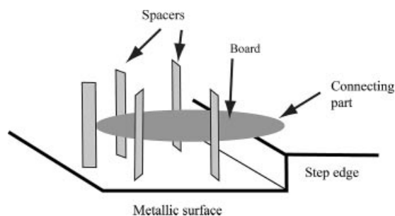
Figure 1. General concept of a 2D-lander connected at the step edge of a metallic surface.
