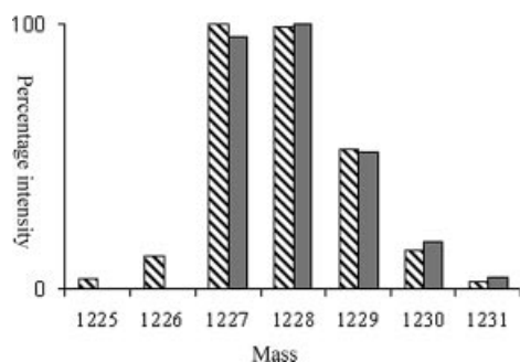
Figure 3. Comparison of the experimental (dashed bars) and calculated (grey bars) DCI mass spectrum (parent ion [M]^+ ) of compound 1 .
